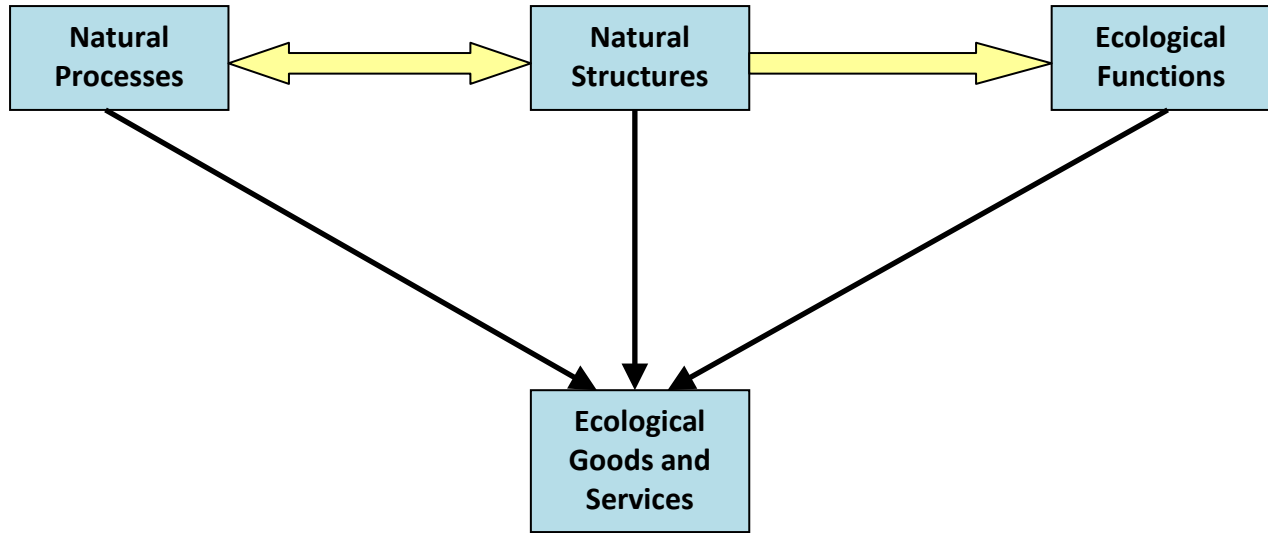
Figure 1. Conceptual Model of Linkages between Processes, Structures, and Functions and Ecological Goods and Services.
